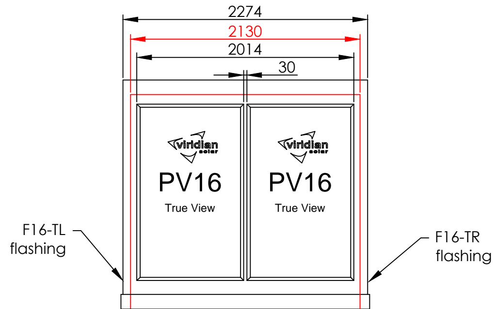
Close-coupled pair of panels 2274mm
