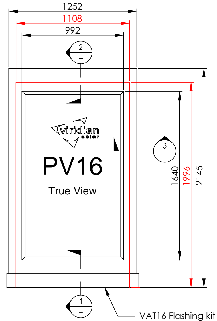
Height for Single Row of Fusion - 2145mm
