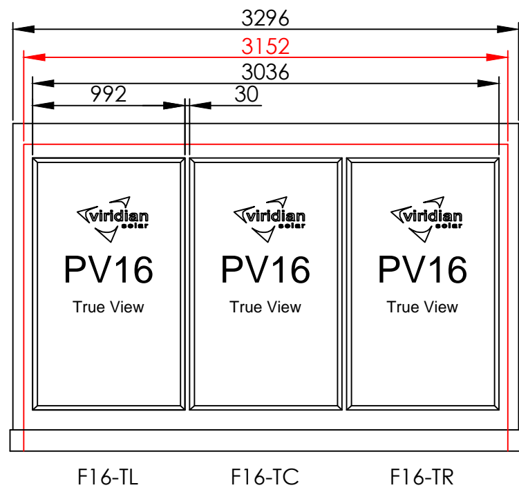
Close-coupled trio of panels 3296mm
